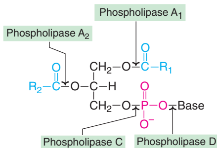
Fig. 14.22 : Degradation of phospholipids by phospholipases.
