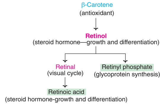
Fig. 7.3 : Summary of the functions of vitamin A compounds.
