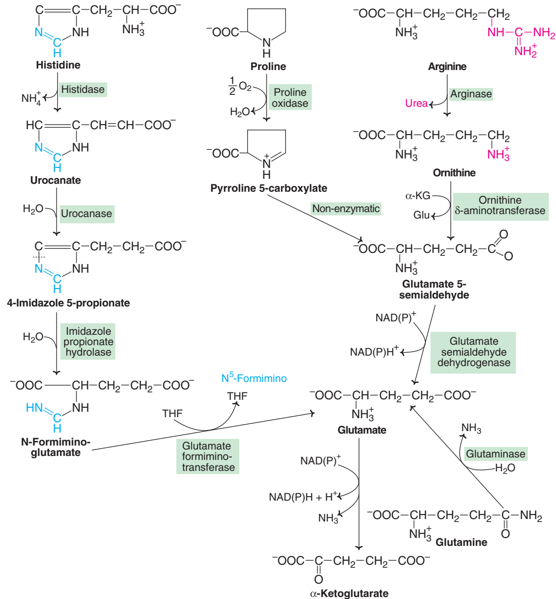
Fig. 15.34 : Metabolism of histidine, proline, arginine, glutamate and glutamine (THF–Tetrahydrofolate; \alpha -KG– \alpha -Ketoglutarate; Glu–Glutamate).
