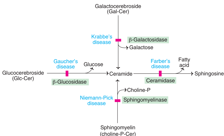
Fig. 14.25 : Degradation of cerebroside and sphingomyelin with metabolic disorders.
