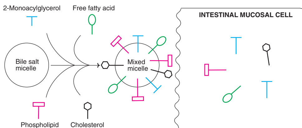
Fig. 8.12 : Absorption of lipids by intestinal mucosal cell.
