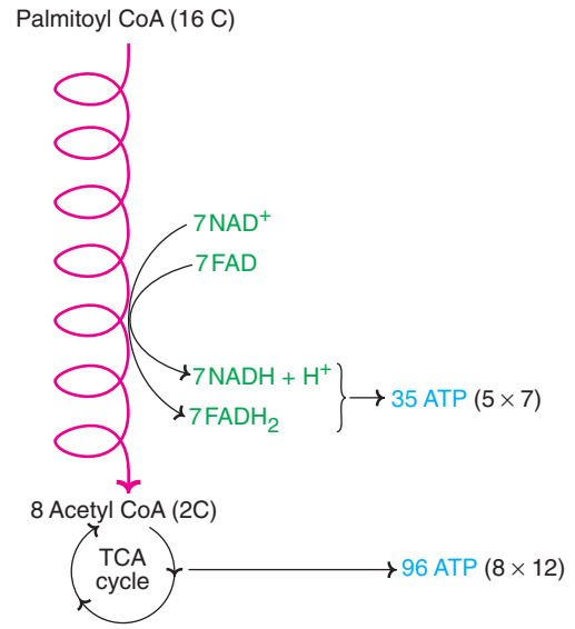
Fig. 14.8 : An overview of oxidation of palmitic acid.
