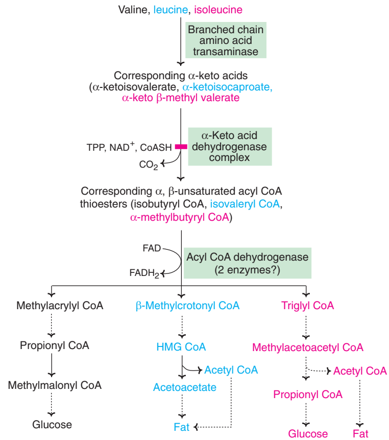
Fig. 15.33 : Summary of branched chain amino acid metabolism (■—Defect in \alpha -keto acid dehydrogenase results in maple syrup urine disease; HMG CoA— \beta -Hydroxy \beta -methyl-glutaryl CoA; Valine is glycogenic, leucine is ketogenic, while isoleucine is both).
