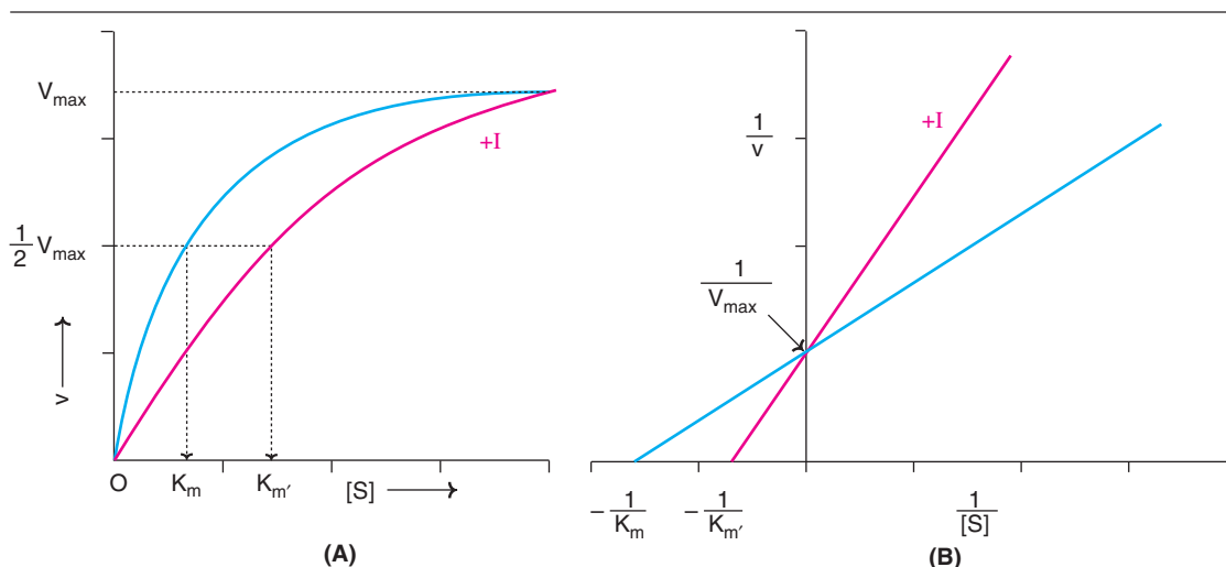
Fig. 6.8 : Effect of competitive inhibitor (i) on enzyme velocity. (A) Velocity (v) versus substrate (S) plot. (B) Lineweaver-Burk plot (Red lines with inhibitor; competitive inhibitor increases K_m' , unalters V_{max} ).
