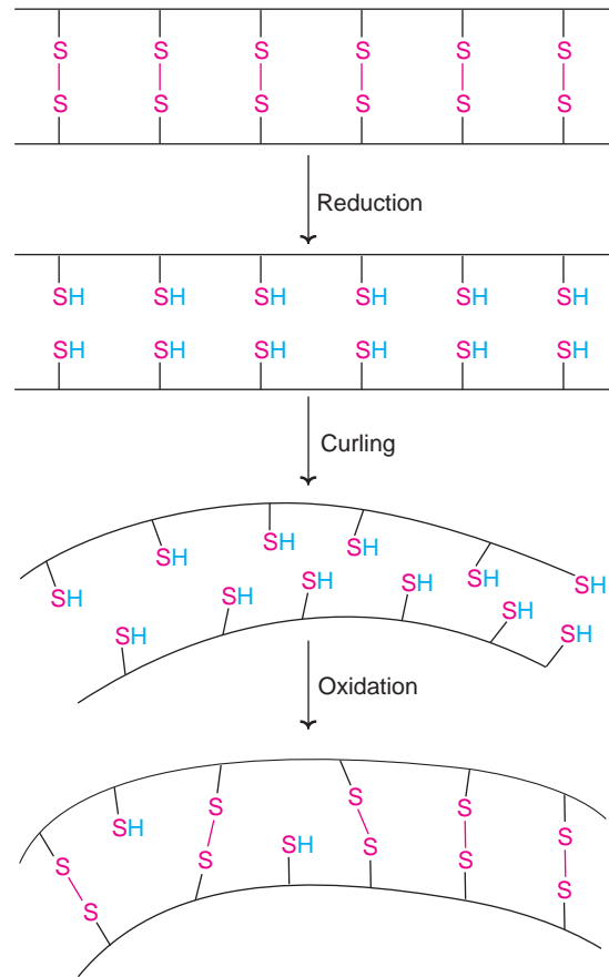
Fig. 22.2 : A diagrammatic representation of hair waving with suitable alterations in keratin structure ( -S-S corresponds to disulfide bonds of cystine; -SH indicates sulfhydryl groups of cysteine)
