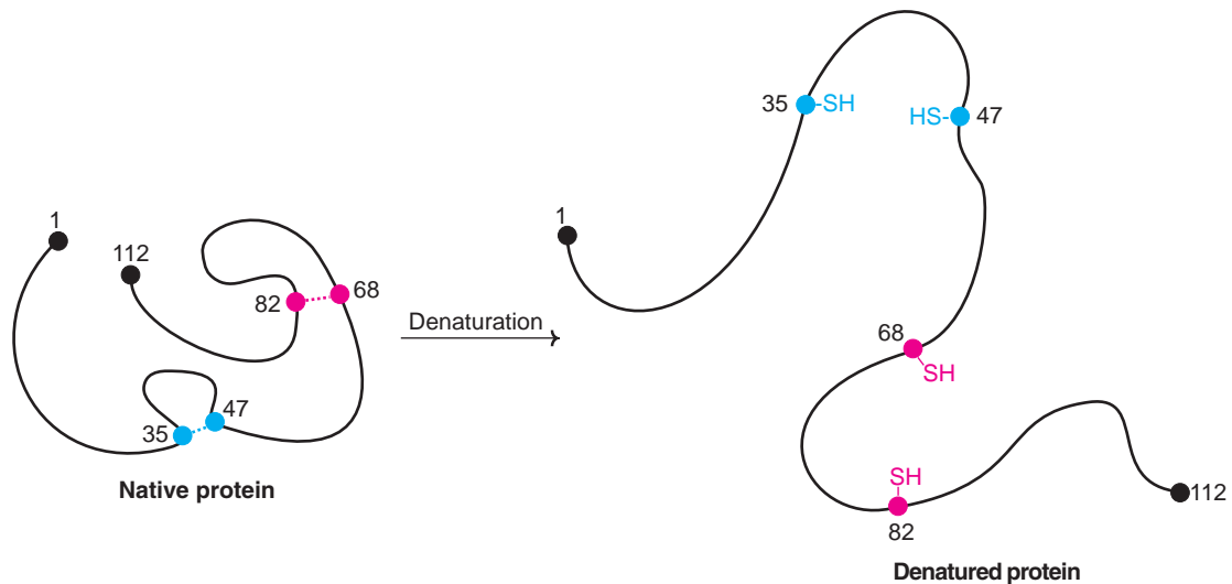
Fig. 4.14 : Denaturation of a protein.
