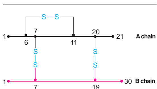
Fig. 4.13 : Diagrammatic representation of human insulin structure (Note : A and B polypeptide chains are held by two disulfide linkages).
