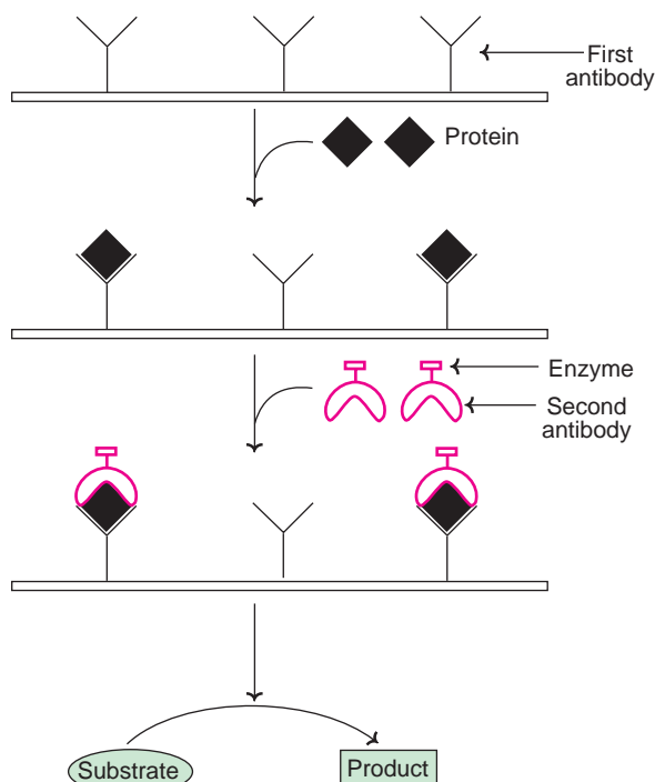
Fig. 41.11 : Diagrammatic representation of enzyme-linked immunosorbant assay (ELISA).
