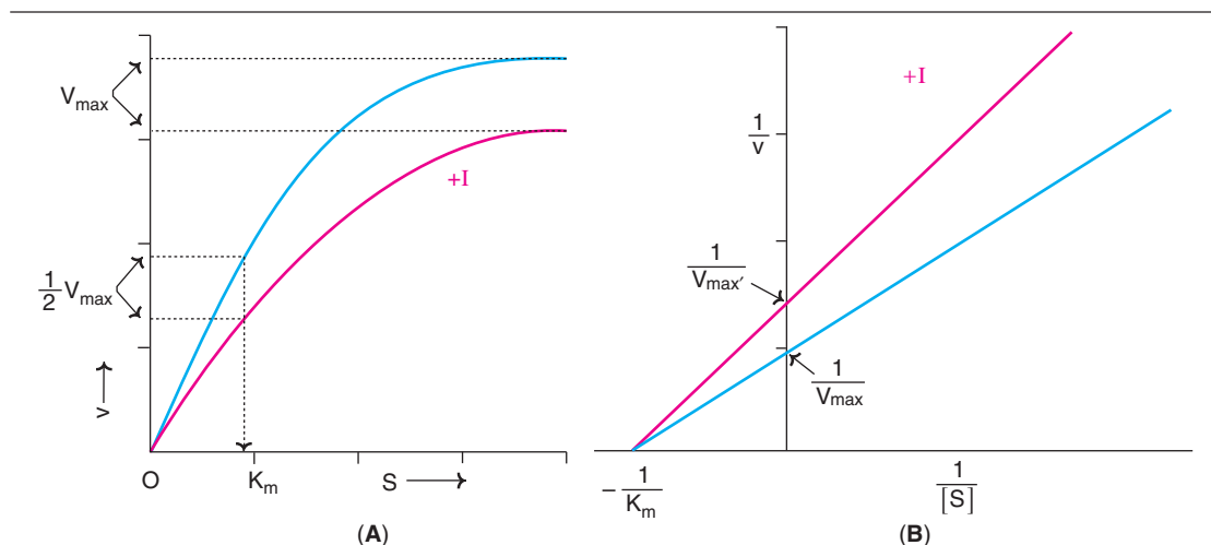
Fig. 6.9 : Effect of non-competitive inhibitor (I) on enzyme velocity (A) Velocity ( v ) versus substrate (S) (B) Lineweaver-Burk plot (Red lines with inhibitor, non-competitive inhibitor does not change K_m but decreases V_{max} ).
