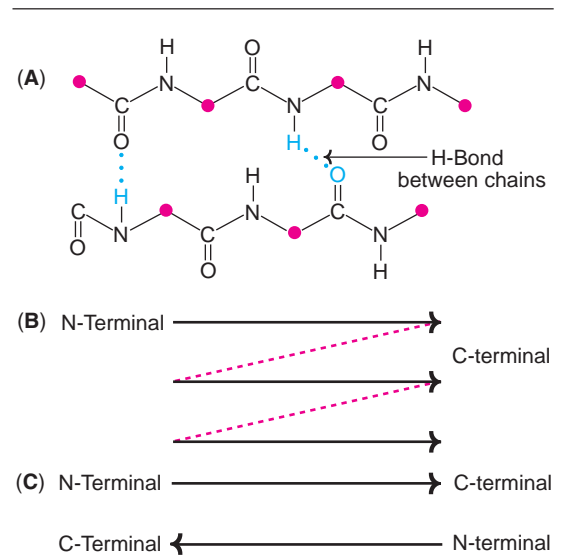
Fig. 4.10 : Structure of \beta -pleated sheet (A) Hydrogen bonds between polypeptide chains (B) Parallel \beta -sheet (C) Antiparallel \beta -sheet. (Note : Red circles in A represent amino acid skeleton— \begin{matrix} \text{H} \\ | \\ \text{—C—R} \end{matrix} ).
