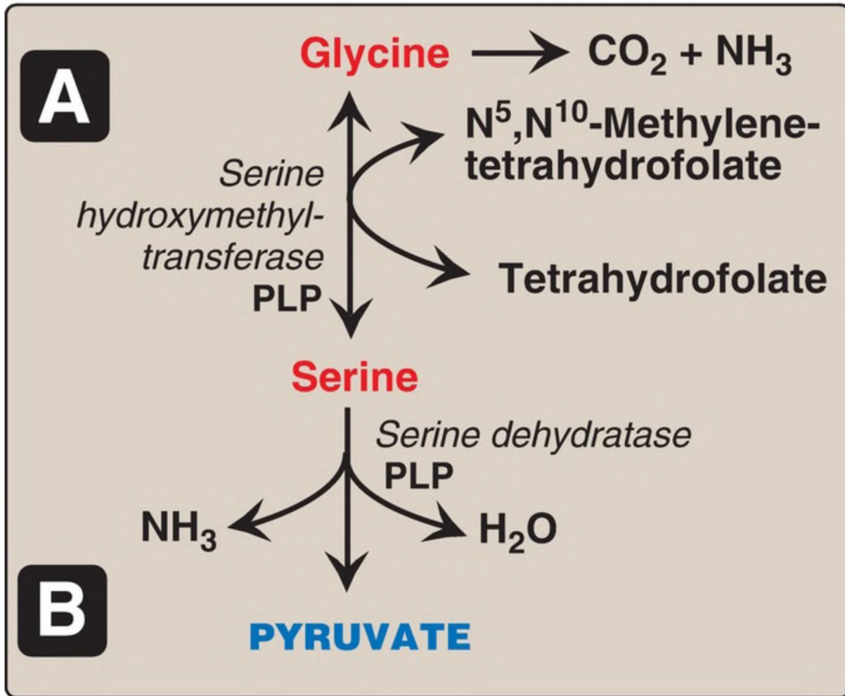
Figure 20.6 A. Interconversion of serine and glycine and oxidation of glycine. B. Dehydration of serine to pyruvate. PLP = pyridoxal phosphate; NH 3 = ammonia.
