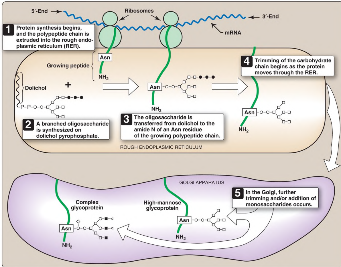
Figure 14.16 Synthesis of N-linked glycoproteins. \circ = N-acetylglucosamine; \square = mannose; \bullet = glucose; \blacksquare = galactose; \diamond or \blacktriangleleft = terminal group (fucose or N-acetylneuraminic acid); mRNA = messenger RNA; Asn = asparagine.
