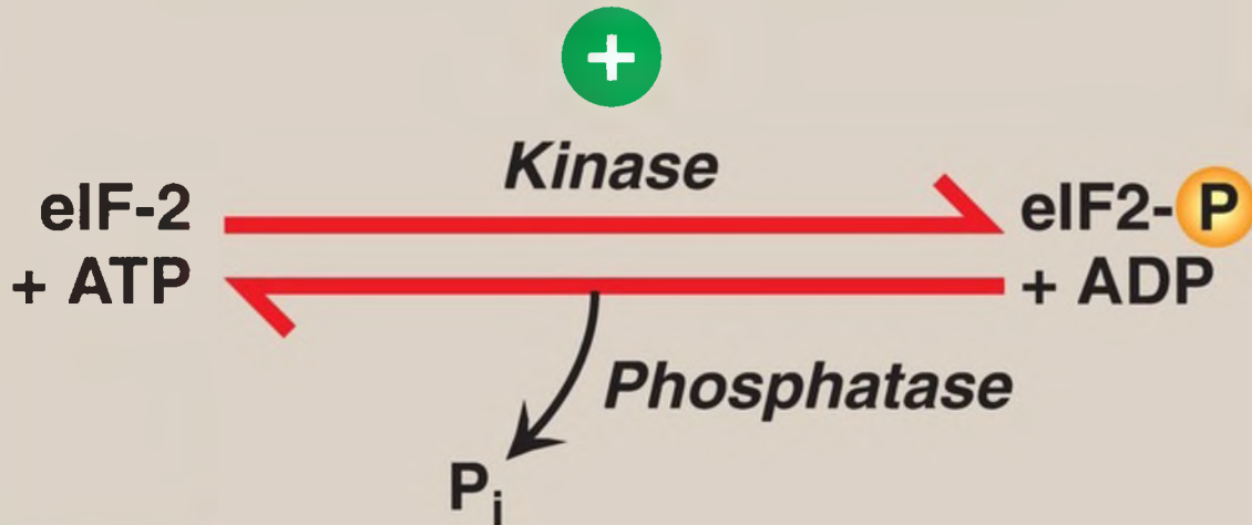
Figure 33.16 Regulation of translation initiation in eukaryotes by phosphorylation of eukaryotic translation initiation factor, eIF-2. RER = rough endoplasmic reticulum; ADP = adenosine diphosphate; P i = inorganic phosphate; = phosphate.
