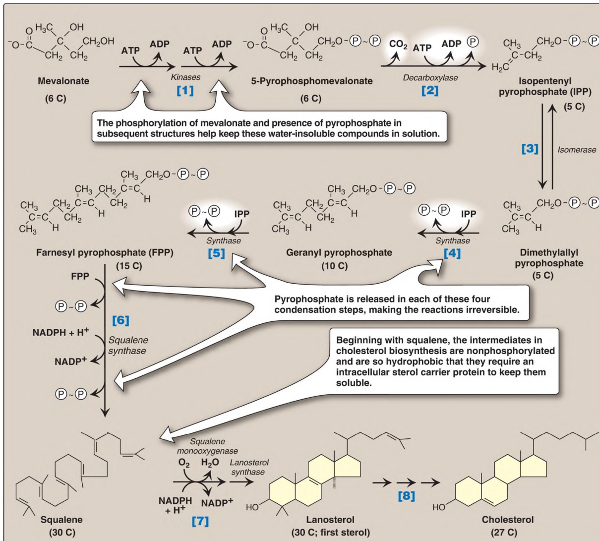
Figure 18.5 Synthesis of cholesterol from mevalonate. ADP = adenosine diphosphate; = phosphate; ~ = pyrophosphate; NADP(H) = nicotinamide adenine dinucleotide phosphate.
