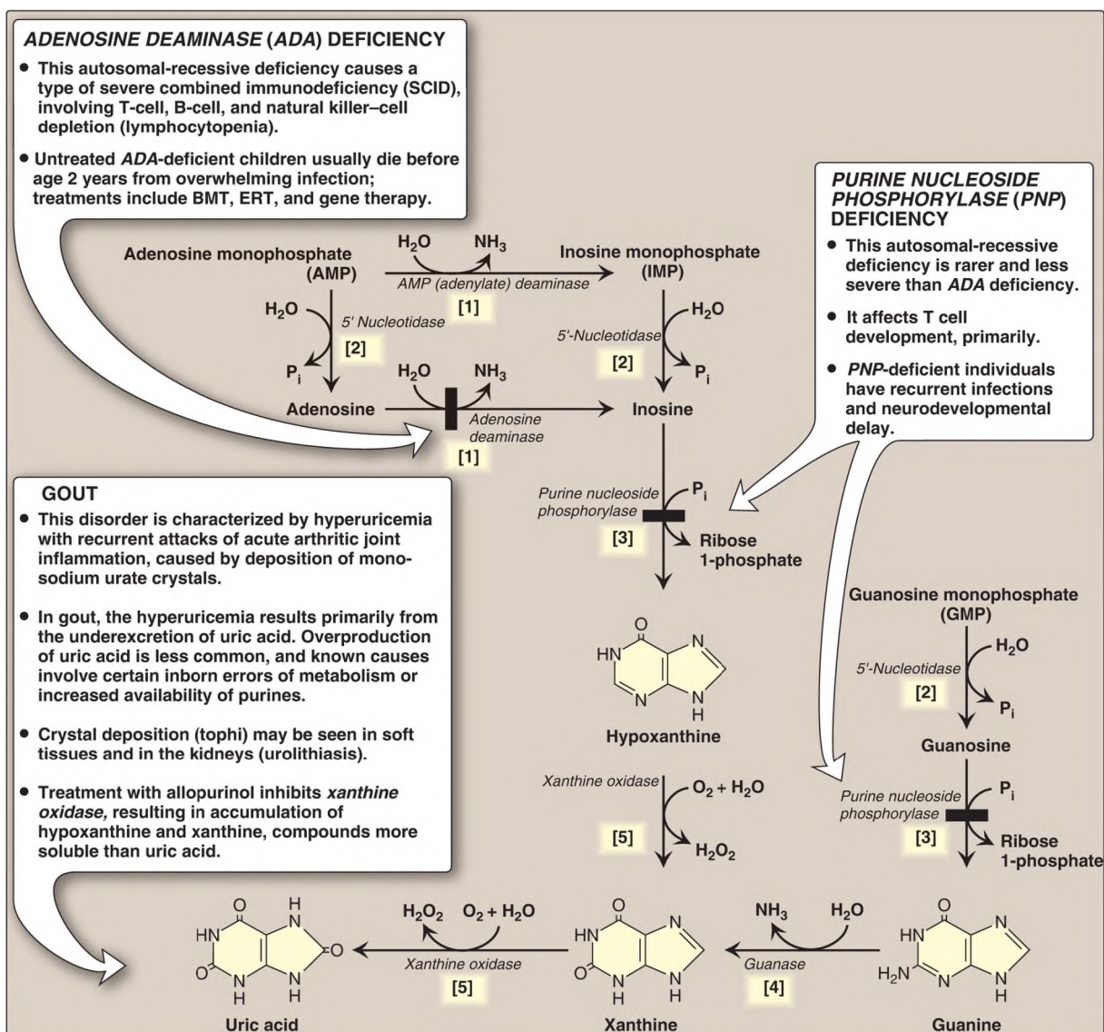
Figure 22.15 The degradation of purine nucleotides to uric acid, illustrating
