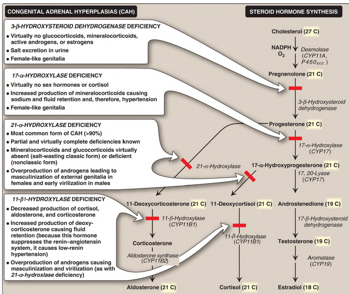
Figure 18.25 Steroid hormone synthesis and associated diseases. [Note: 3-β-Hydroxysteroid dehydrogenase , CYP17 , and CYP11B2 are multifunctional enzymes. Synthesis of testosterone and the estrogens occurs primarily outside of the adrenal gland.] NADPH = nicotinamide adenine dinucleotide phosphate; CYP = cytochrome P450.
