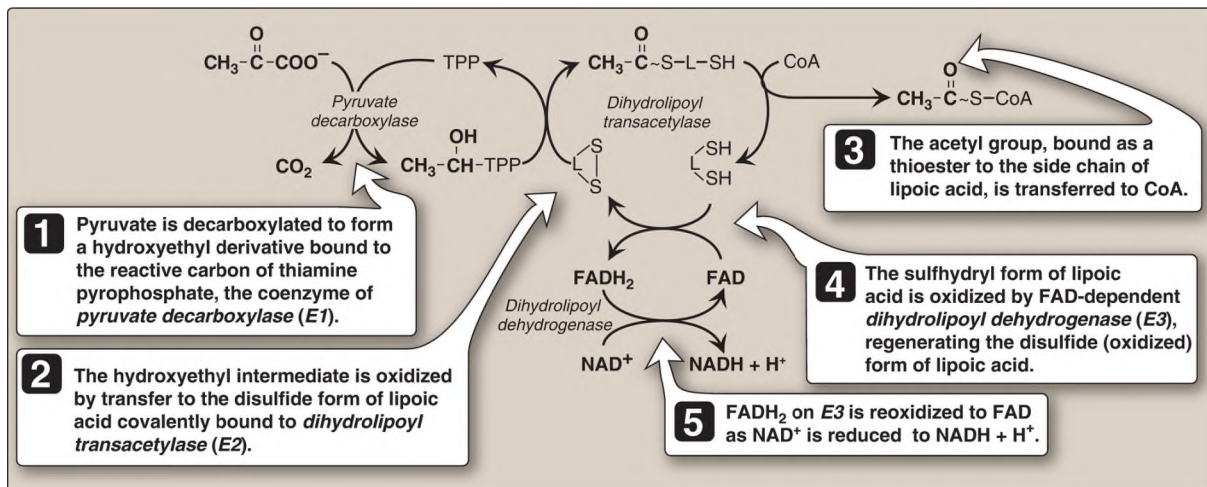
Figure 9.2 Mechanism of action of the enzymes ( E ) of the pyruvate dehydrogenase complex . [Note: All the coenzymes of the complex, except for lipoic acid, are derived from vitamins. TPP is from thiamine, FAD from riboflavin, NAD from niacin, and CoA from pantothenic acid.] CO 2 = carbon dioxide; TPP = thiamine pyrophosphate; L = lipoic acid; CoA = coenzyme A; FAD(H 2 ) and NAD(H) = flavin and nicotinamide adenine dinucleotides; ~ = high-energy bond.
