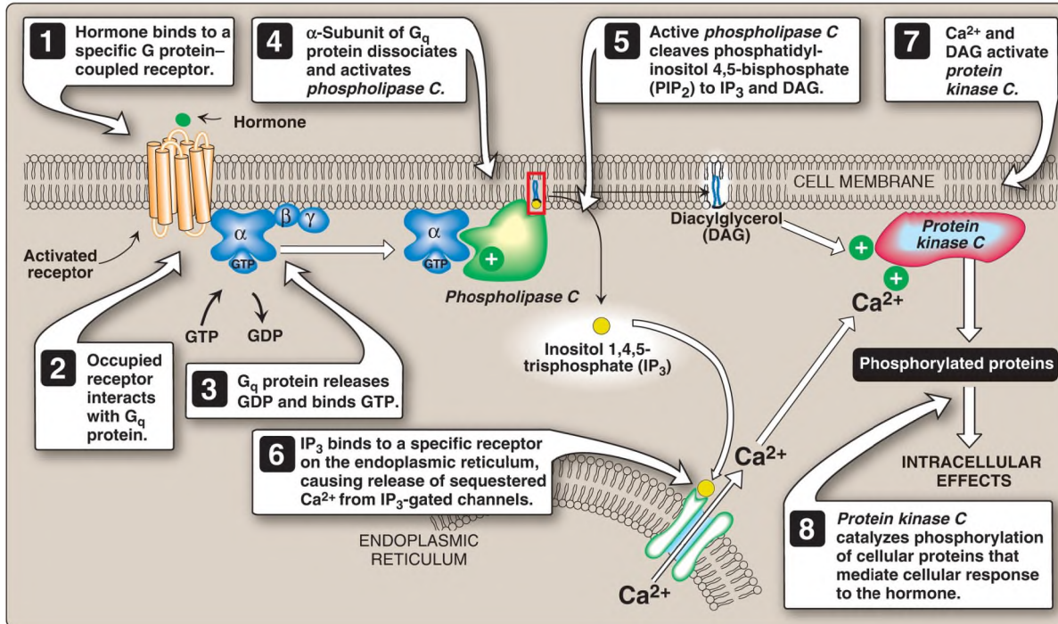
Figure 17.8 Role of inositol triphosphate and diacylglycerol in cell signaling. GDP and GTP = guanosine di- and triphosphates; Ca 2+ = calcium.
