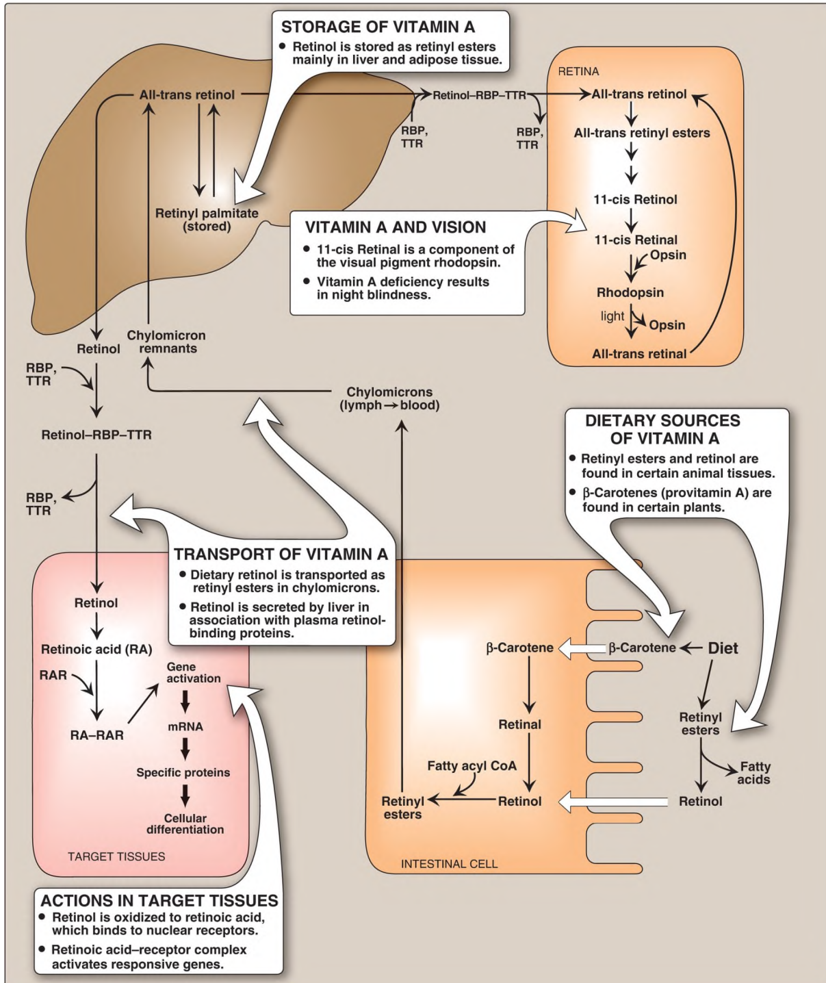
Figure 28.19 Absorption, transport, and storage of vitamin A and its derivatives. [Note: \beta -Carotene is a carotenoid, a plant pigment with antioxidant activity.] RBP = retinol binding protein; TTR = transthyretin; RAR = retinoic acid receptor; CoA = coenzyme A; mRNA = messenger RNA.
