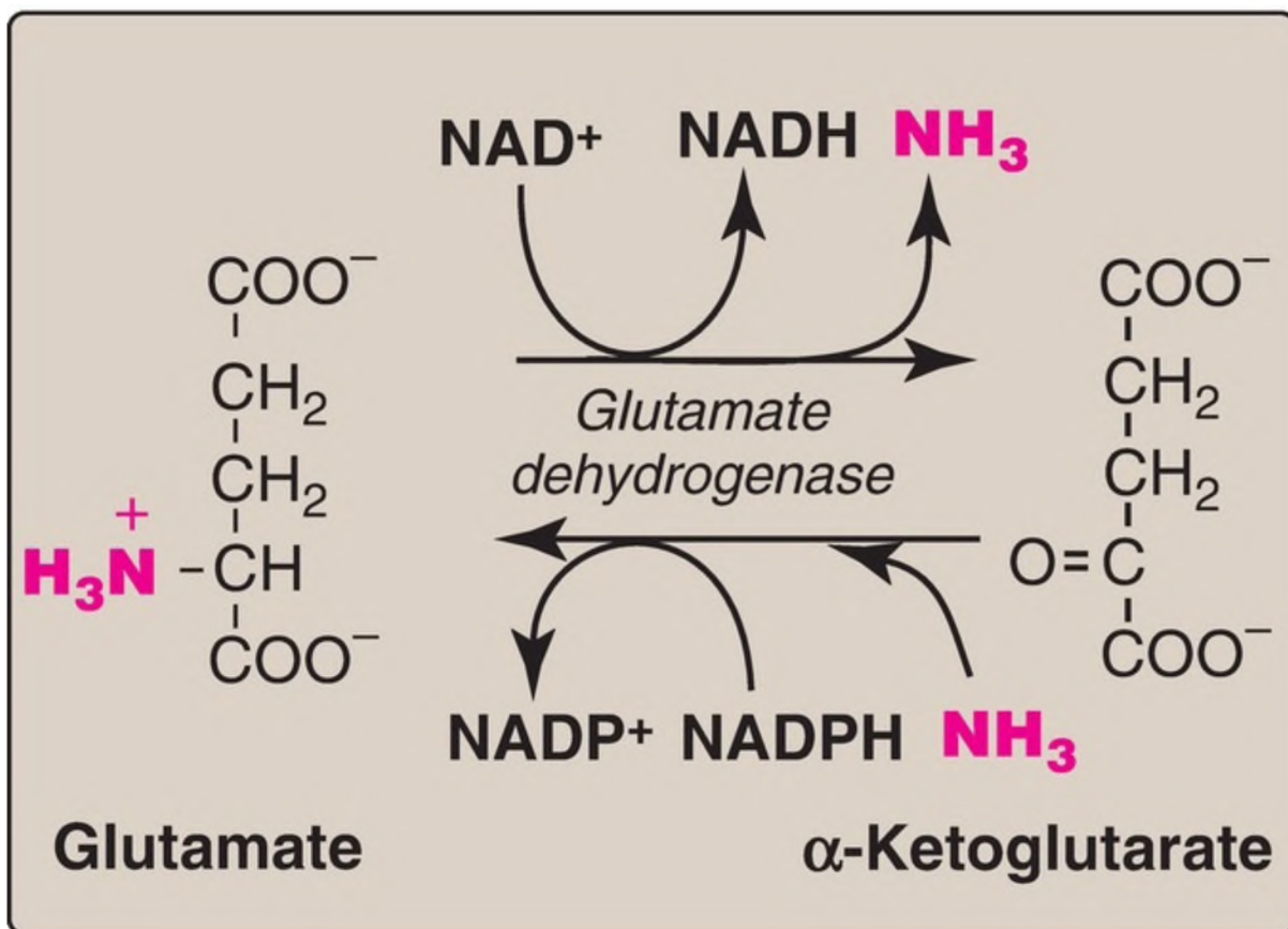
Figure 19.11 Oxidative deamination by glutamate dehydrogenase . [Note: The enzyme is unusual in that it uses both \text{NAD}^+ (nicotinamide adenine dinucleotide) and \text{NADPH} (nicotinamide adenine dinucleotide phosphate).] \text{NH}_3 = ammonia.
