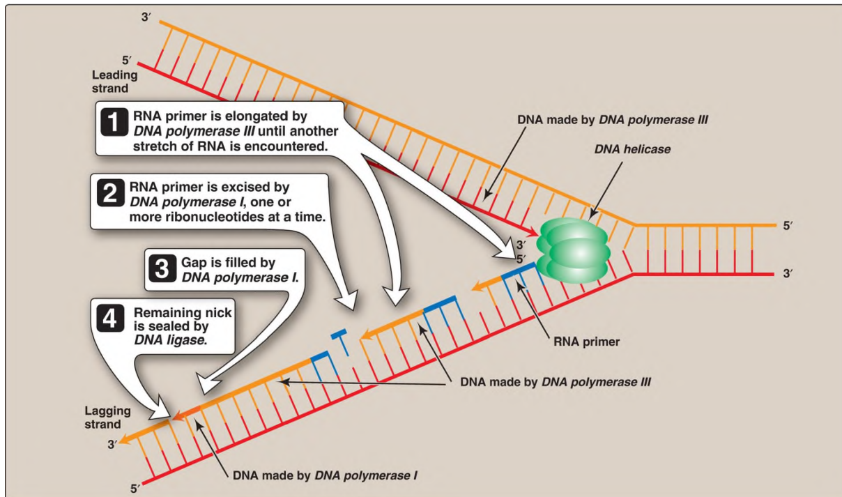
Figure 30.19 Removal of RNA primer and filling of the resulting gaps by DNA polymerase I .
