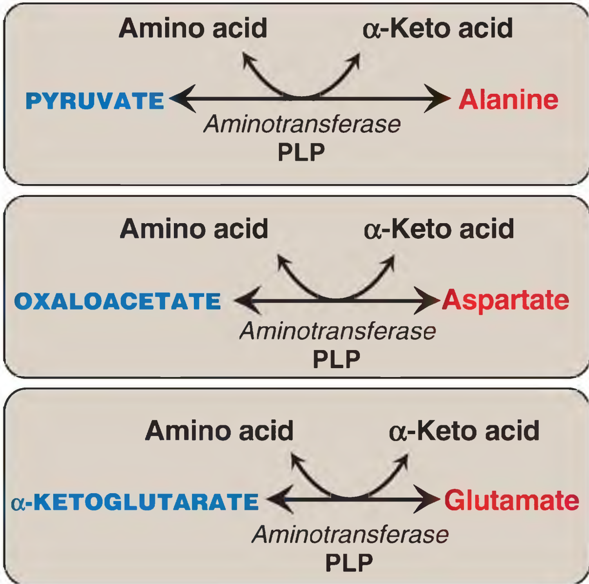
Figure 20.13 Formation of alanine, aspartate, and glutamate from the corresponding α-keto acids by transamination. PLP = pyridoxal phosphate.
