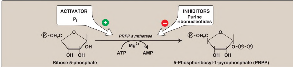
Figure 22.6 Synthesis of PRPP, showing the activator and inhibitors of the reaction. [Note: This is not the committed step of purine synthesis because PRPP is used in other pathways such as salvage (see p. 296).] = phosphate; P i = inorganic phosphate; AMP = adenosine monophosphate; Mg = magnesium.
