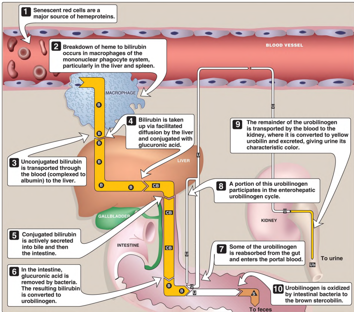
Figure 21.10 Catabolism of heme. = bilirubin; = conjugated bilirubin; = urobilinogen; = urobilin; = stercobilin.
